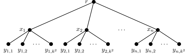
Figure 3: The constructed tree T . The labels of the vertices are: l(r) = a(S) and l(x_i) = a(s_i) - a(S)/(k - 1) .
