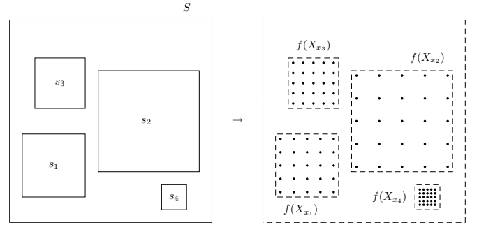
Figure 4: The embedding constructed for the YES instance.
